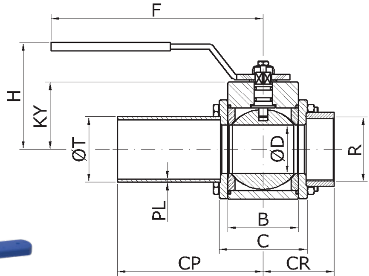
WELDING JOINT
